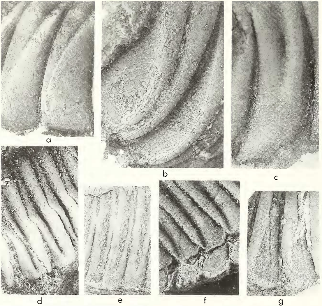
TEXT-FIG. 13. The petaloid thoracic facet ( a and b ), typical of higher Asaphina, compared with facets of other trilobites ( c-g ). a , asaphid, Asaphus sp. BM 15430 (Middle Ordovician, Russia), \times 8 . b , nileid, Symphysurus palpebrosus , BM It20684 (Middle Ordovician, Sweden), \times 8 . c , granulose dalmanitacean facet, Dalmanites caudatus , BM I67a (Silurian), with postfacetal type of pleural furrow, \times 8 . d , primitive type, smooth, in the Silurian proetide Otarion diffractum , BM I3603, \times 12 . e, f , primitive type in the Middle Cambrian ptychoparioid Elrathia ; e , BM It5396, dorsal surface, \times 12 ; f , BM It5397, narrow double ridge with terrace ridges primitive for Asaphina, \times 15 . g , granulose calymenacean facet, with epifacial type of pleural furrow, Calymene sp., BM It20685 (Upper Ordovician, Anticosti Island), \times 10 .
